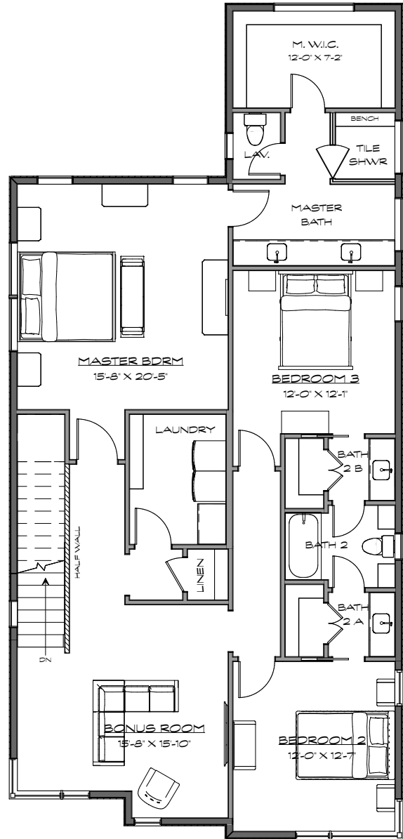
SECOND FLOOR
